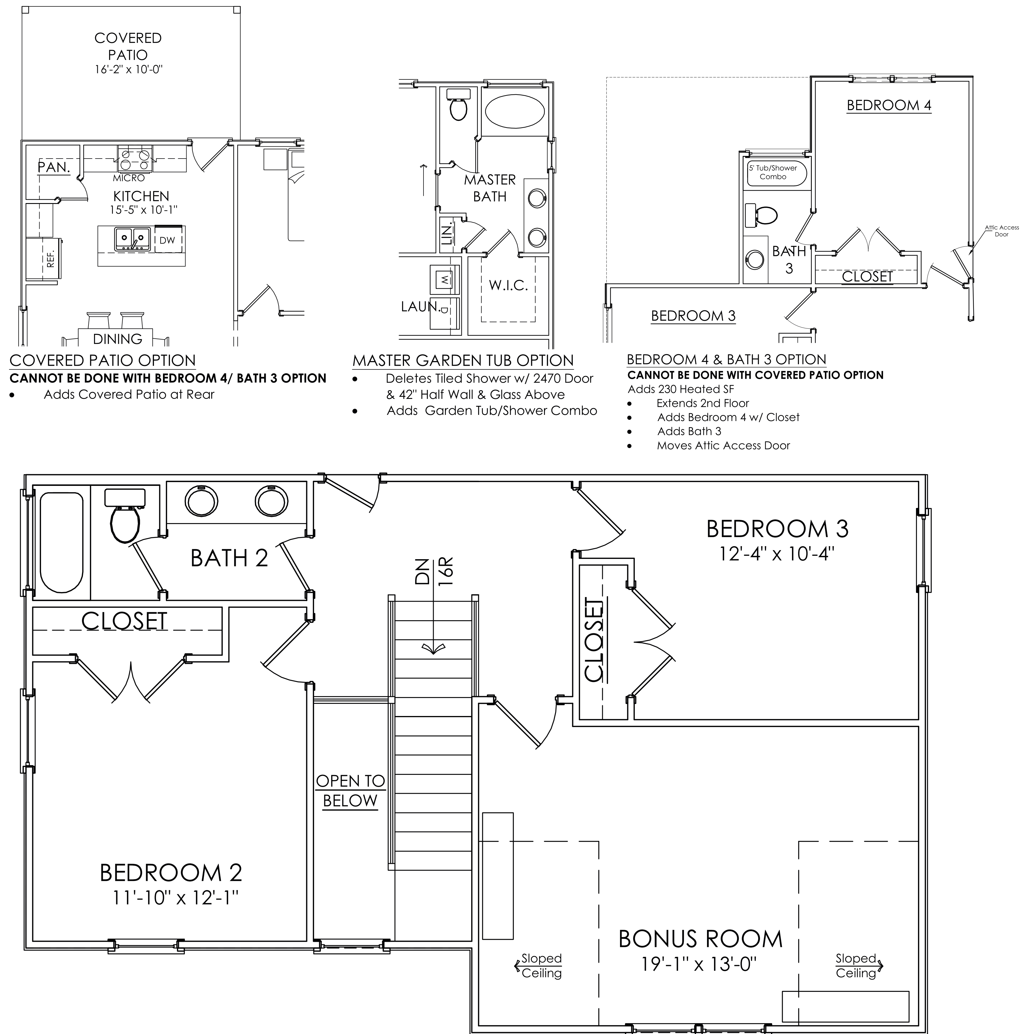
Upper Level Floor Plan
