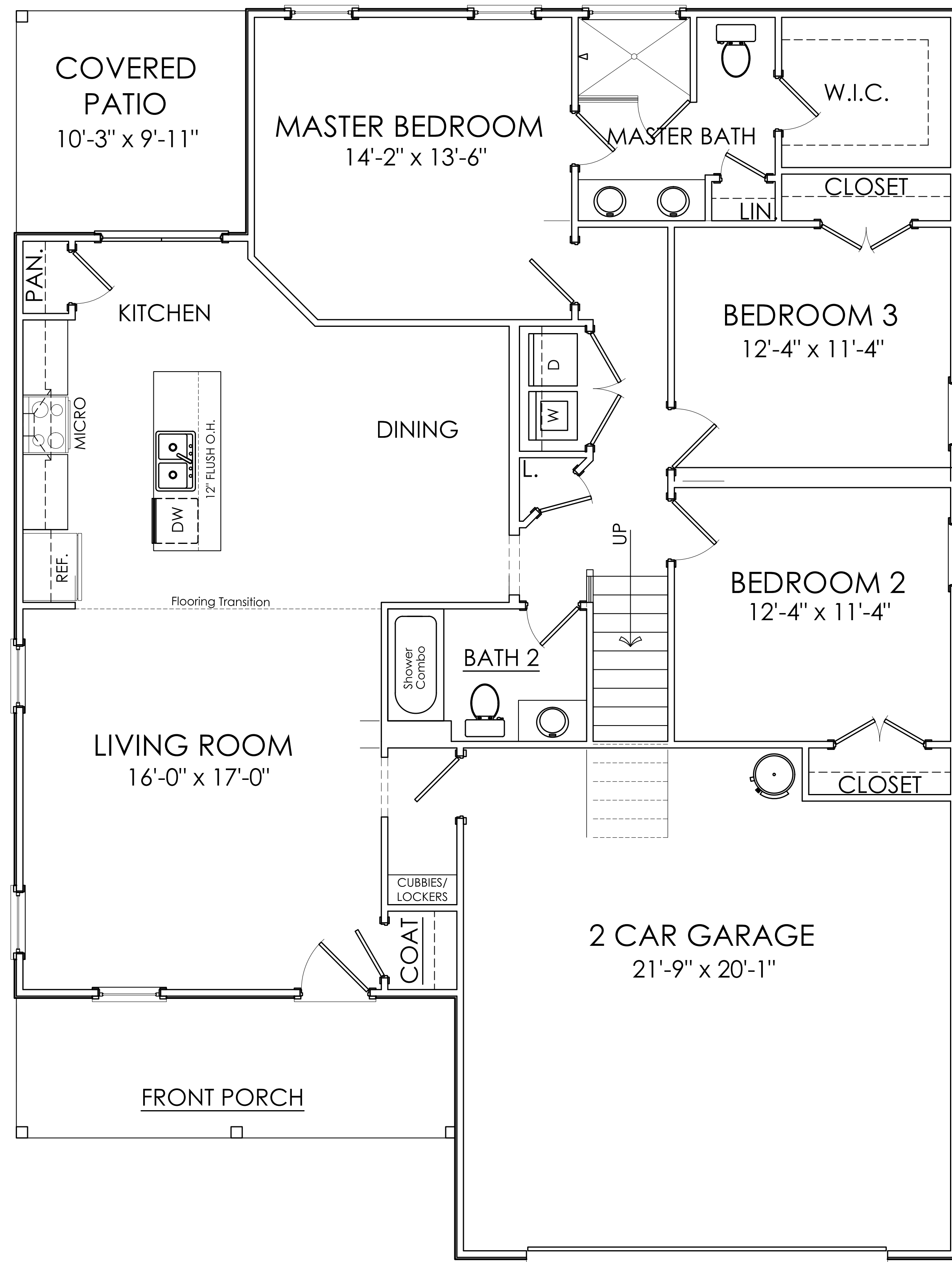
Main Level Floor Plan
