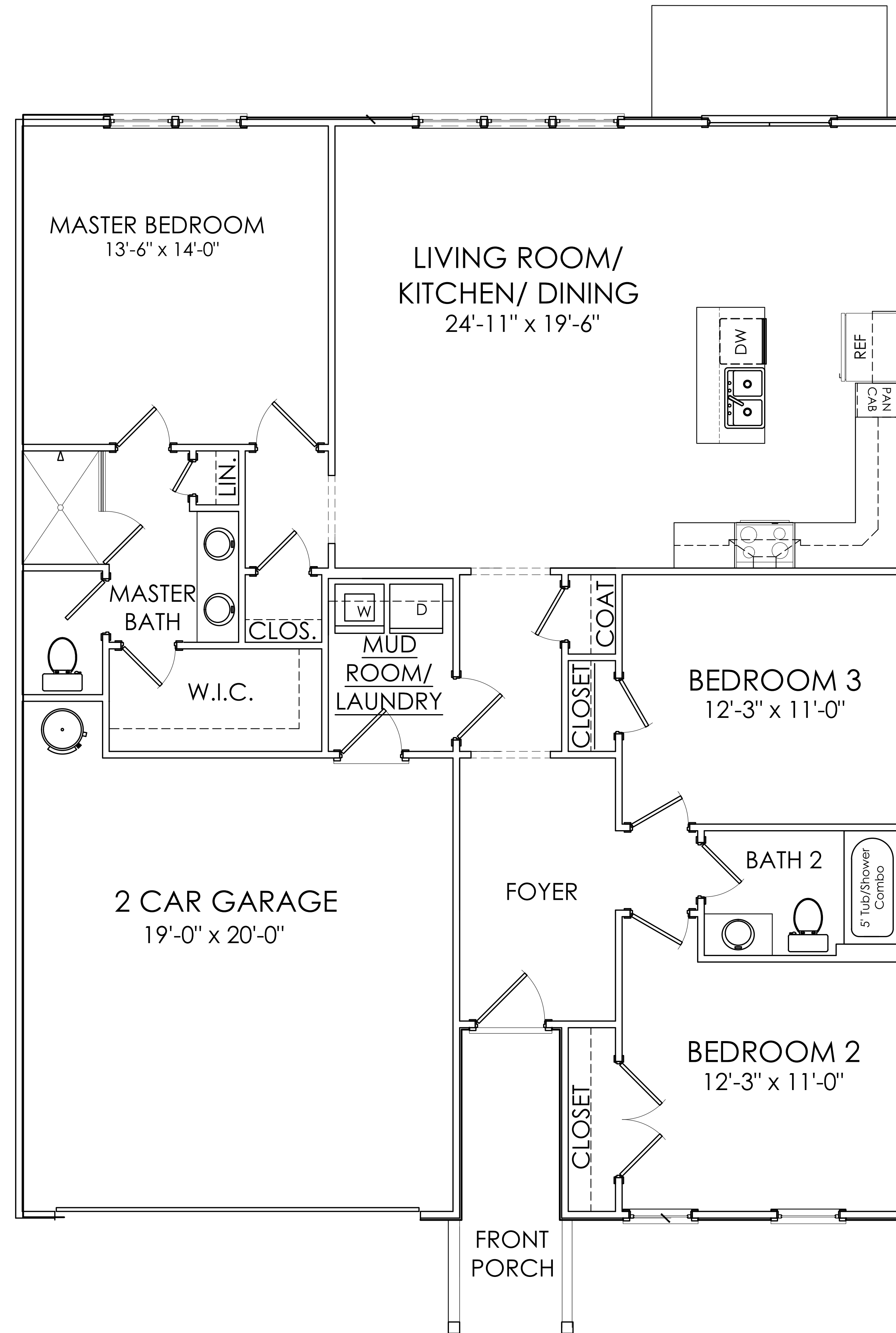
Main Level Floor Plan
